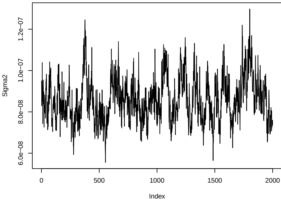
Trace plot of Sigma2
