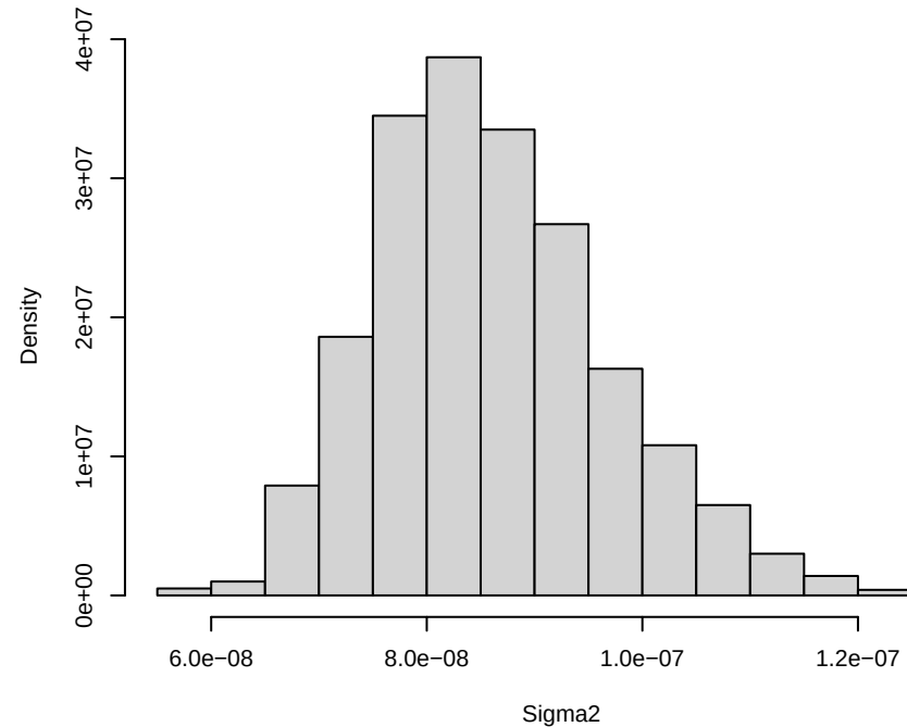
Density of Sigma2
