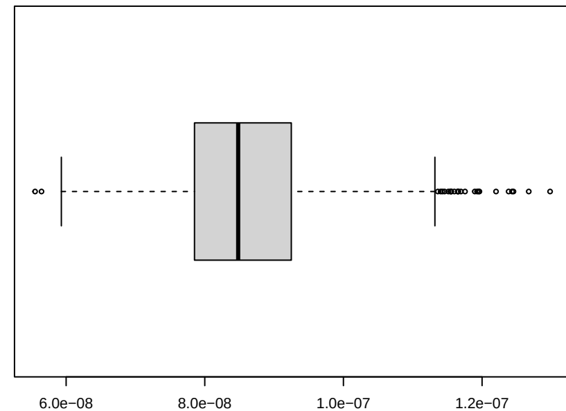
Box plot of Sigma2
